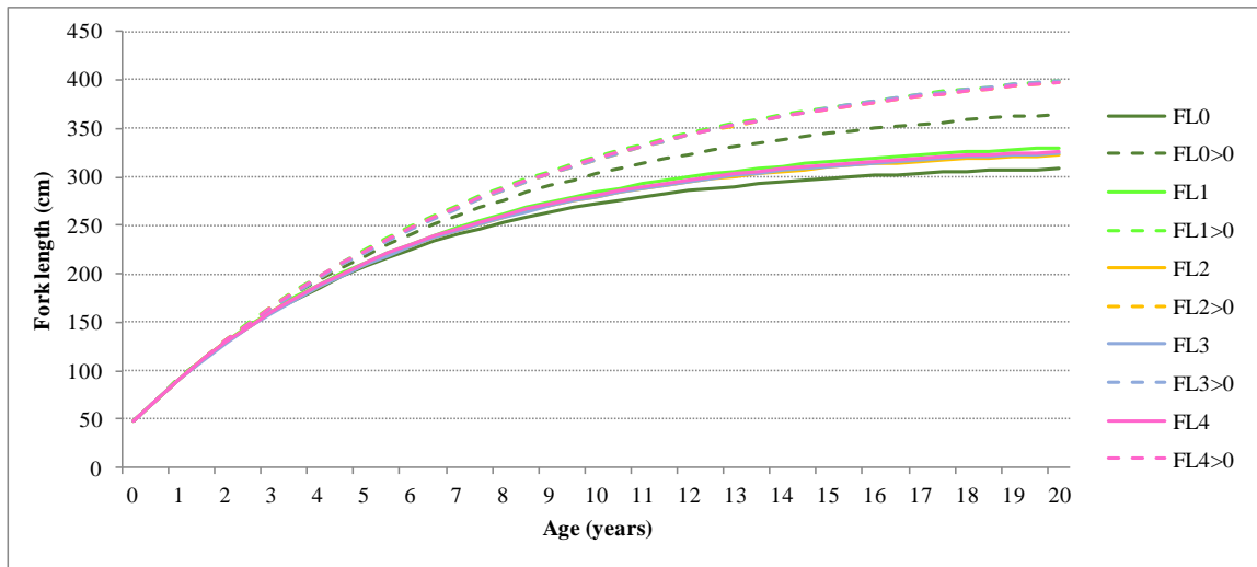
Figure 2. How the TL to FL transformation equation used, or taking into account only records with positive growth without other data cleaning, influence the growth curve. FL0=only records measured in FL units. FL1=transforming TL to FL using Castro and Mejuto (1995) equation. FL2=transforming TL to FL using Campana et al. (2005) equation. FL3=transforming TL to FL using Kohler et al. (1995) equation. FL4=transforming TL to FL using Mas et al. (2014) equation. FLx > 0 using only records with positive growth.
